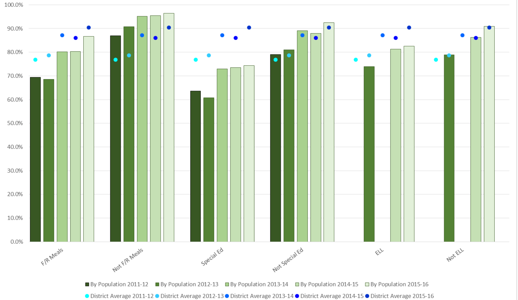
Graduation Rate - Special Populations - 2012-2016
